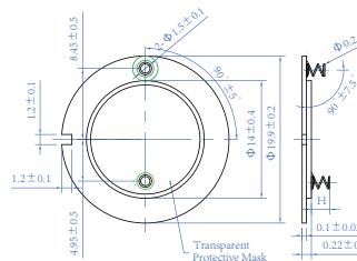
Dimensions (mm)
